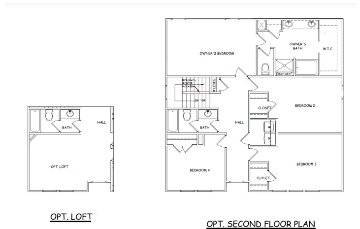
OPT. SECOND FLOOR PLAN
