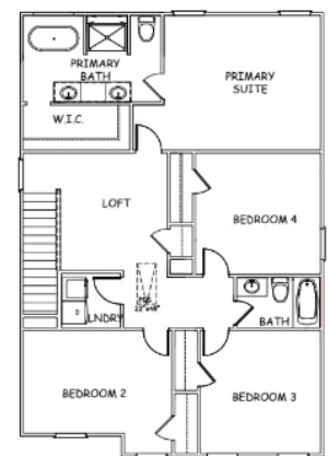
OPT SECOND FLOOR PLAN (SCALE 1/8" = 1')
