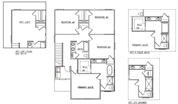
OPT. SECOND FLOOR PLAN (SCALE 3/8" = 1')
