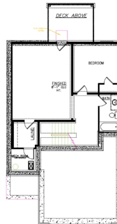
FINISHED BASEMENT PLAN 766 SQ. FT. SCALE 1/8"=1'-0"
