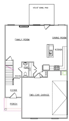
FIRST FLOOR PLAN (SCALE 1/8"=1'-0")
