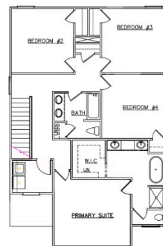
OPT. SECOND FLOOR PLAN (SCALE 1/8"=1'-0")
