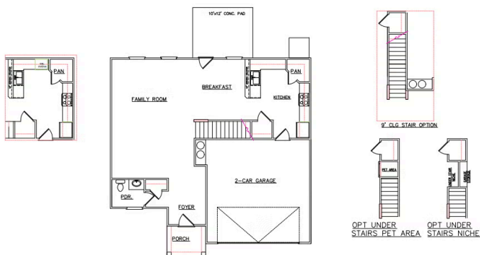
FIRST FLOOR PLAN (BASE OPTION)
