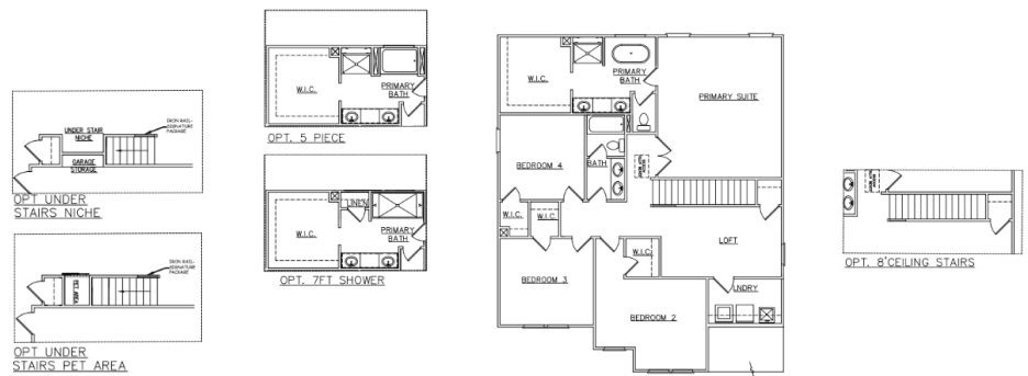
SECOND FLOOR PLAN (SCALE 1/8"=1'-0")
