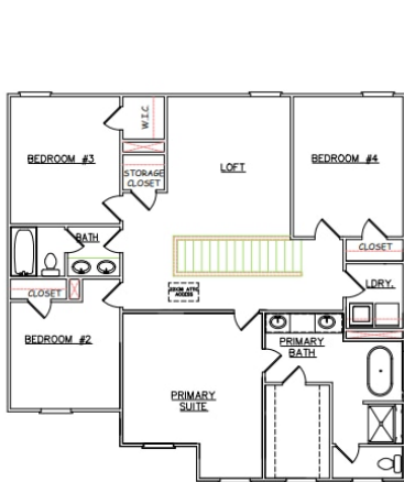
OPT. SECOND FLOOR PLAN
