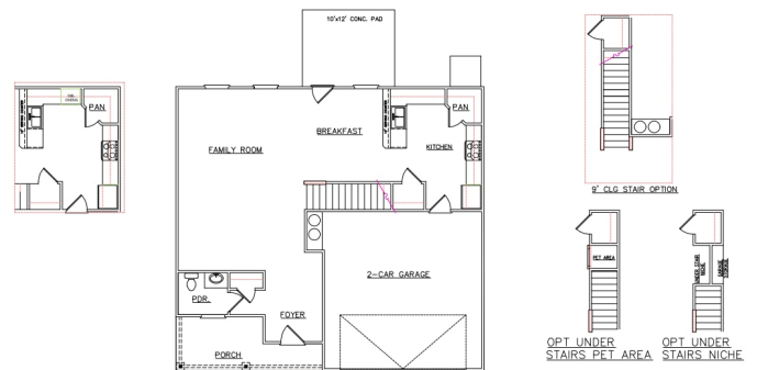
FIRST FLOOR PLAN (SHEET 1010-01)
