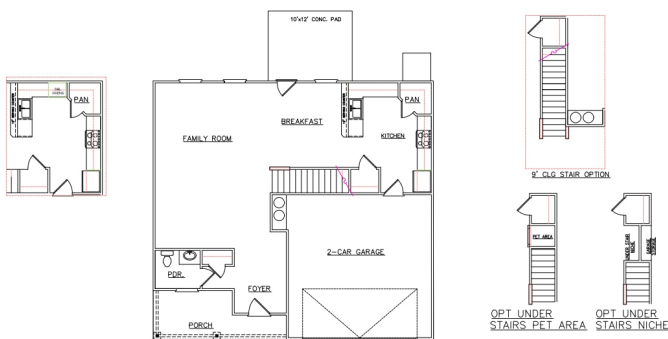
FIRST FLOOR PLAN (BOARD OPTION)
