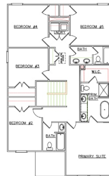
SECOND FLOOR PLAN (SCALE 1/8"=1'-0")
