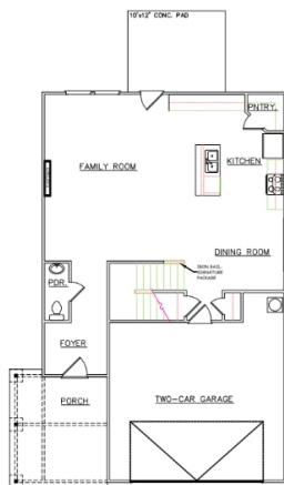
FIRST FLOOR PLAN (SCALE 1/8"=1'-0")
