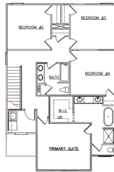
OPT. SECOND FLOOR PLAN (SCALE 1/8" = 1')
