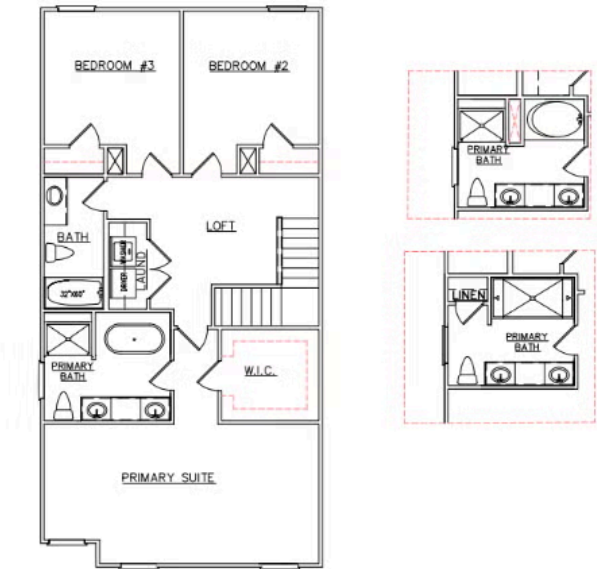
SECOND FLOOR PLAN-NELSON
