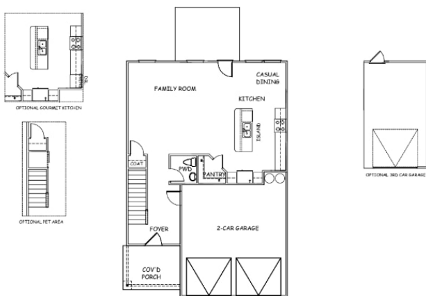
FIRST FLOOR PLAN (SCALE 3/8"=1'-0")
