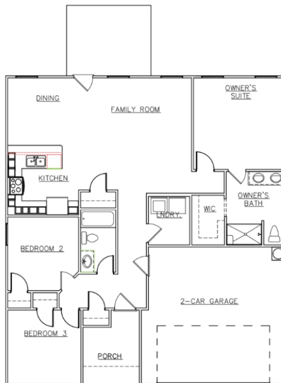
1ST FLOOR
