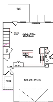
FIRST FLOOR PLAN (SHEET 1 OF 2)
