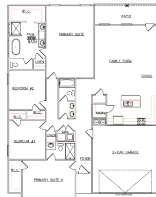
OPT FIRST FLOOR PLAN
