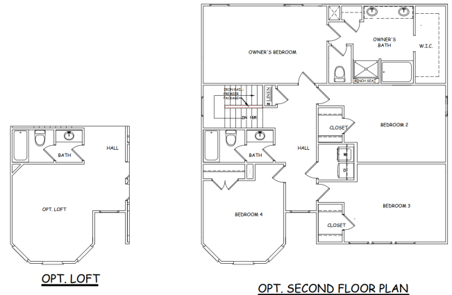
OPT. SECOND FLOOR PLAN
