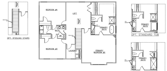
OPT. SECOND FLOOR PLAN (SCALE 1/8" = 1'-0")
