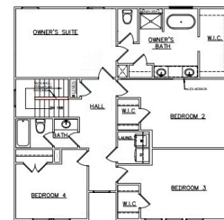
OPT. SECOND FLOOR PLAN
