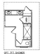
OPT. SECOND FLOOR PLAN (SCALE 1/8"=1'-0")
