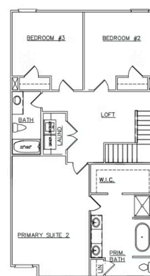
OPT SECOND FLOOR PLAN
