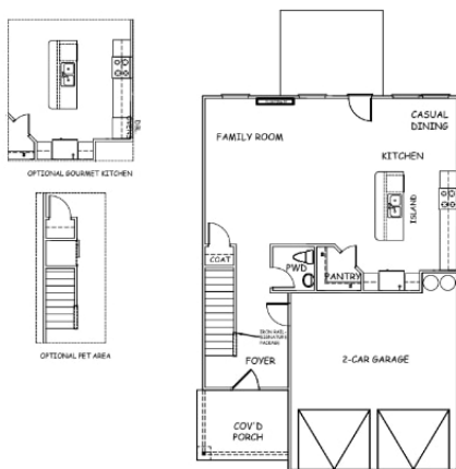
FIRST FLOOR PLAN (SCALE 1/8" = 1')
