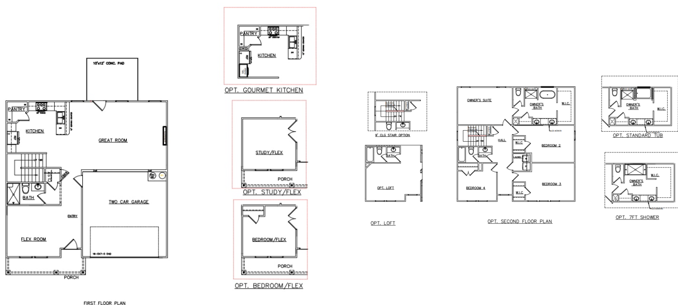
1ST FLOOR
