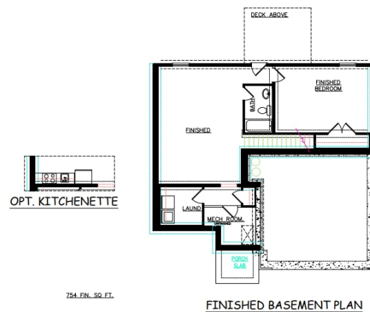
FINISHED BASEMENT PLAN
