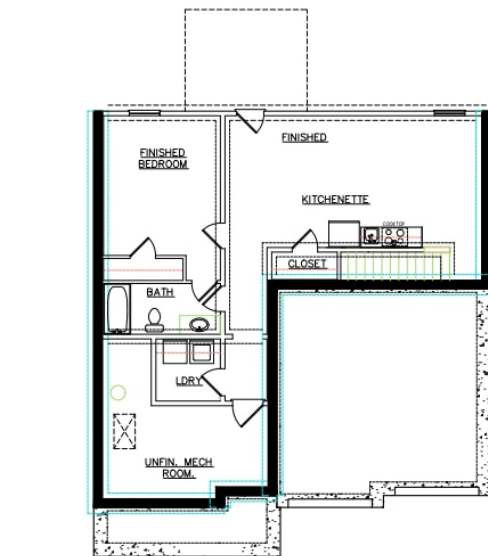
FINISHED BASEMENT (SCALE: 1/8"=1'-0")
