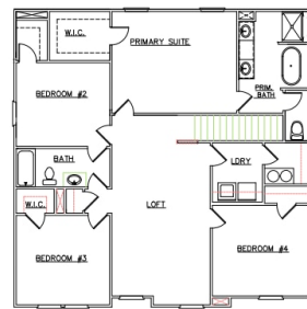
SECOND FLOOR PLAN OPT BATH (SCALE 1/8"=1'-0")
