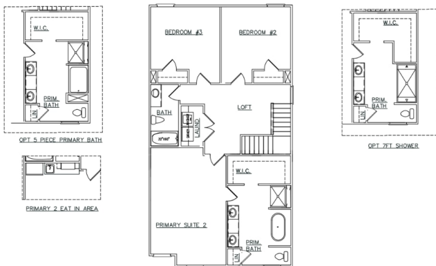
OPT SECOND FLOOR PLAN
