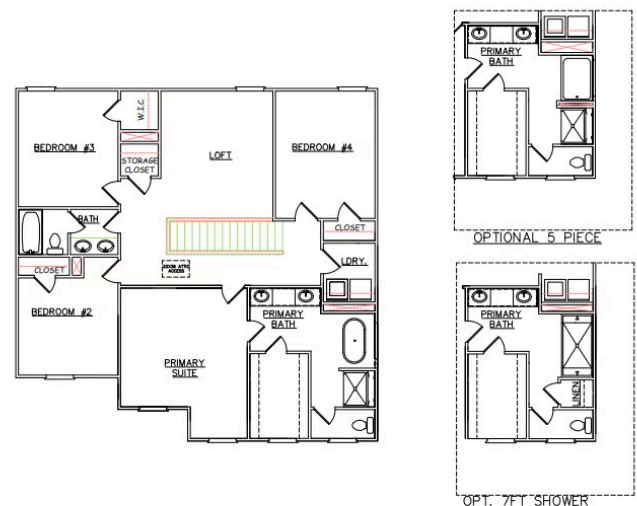
OPT. SECOND FLOOR PLAN
