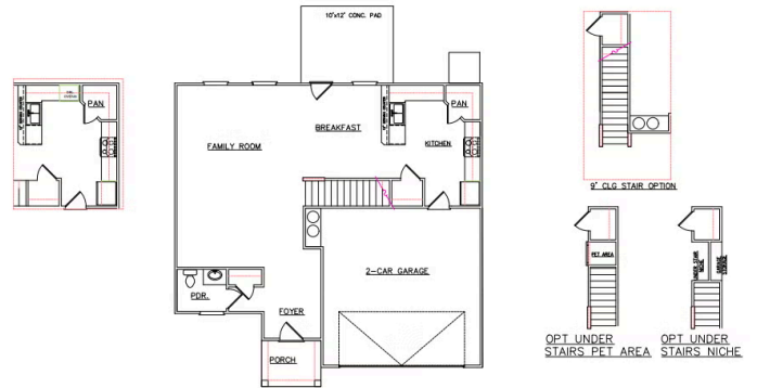
FIRST FLOOR PLAN (SCALE 1/8"=1'-0")
