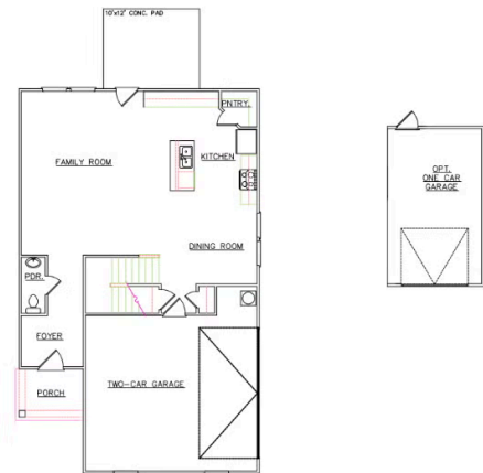
FIRST FLOOR PLAN (SCALE 1/8"=1'-0")
